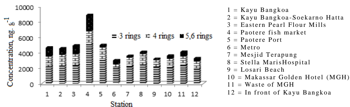
Figure 2. The relative abundance of PAHs compounds in the sediment of Losari Beach and adjacent (Based on the number rings)
